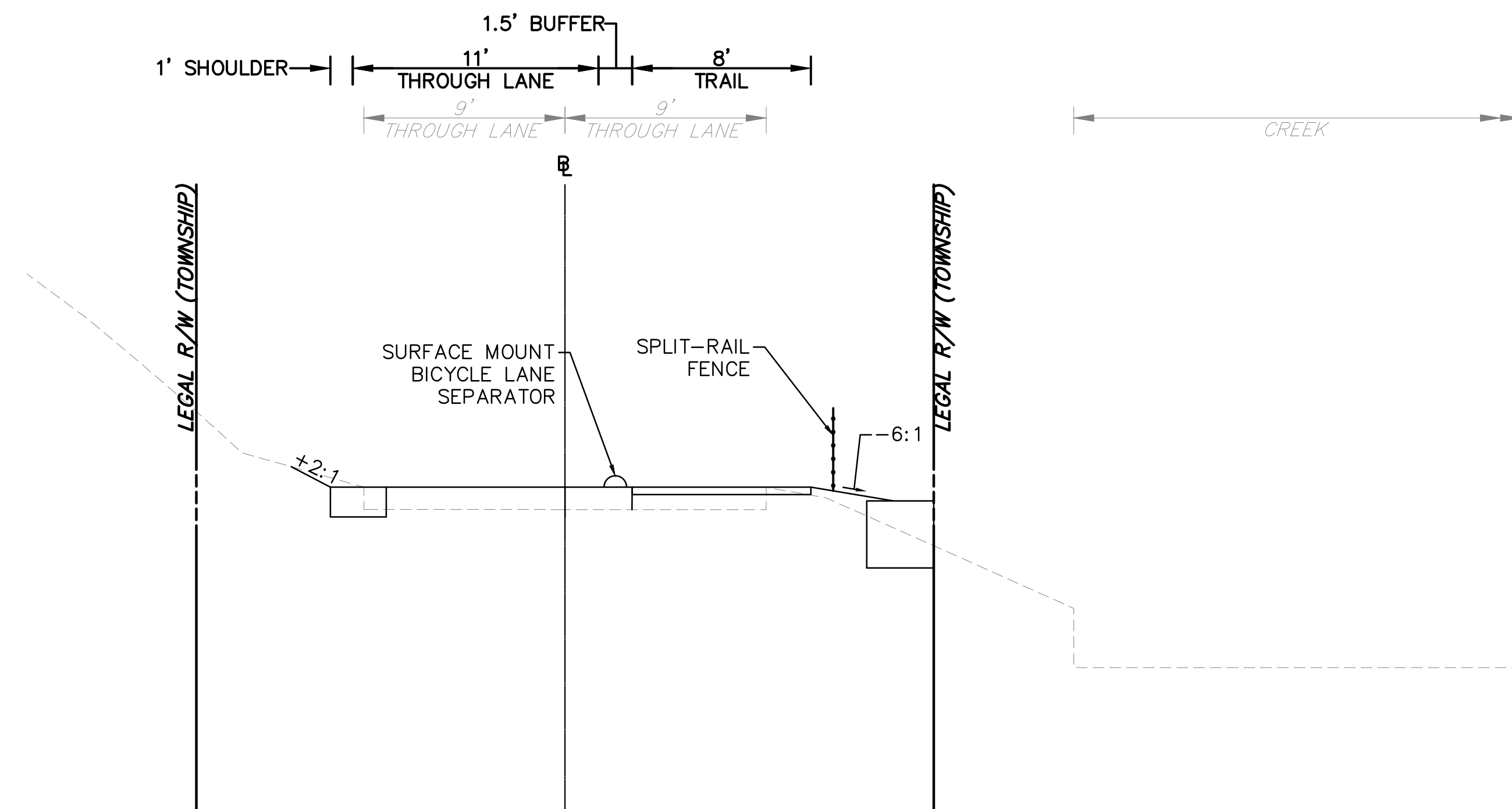
TYPICAL ONE-LANE CHOKER SECTION STA. 13+00 TO STA. 19+00 8' TRAIL
