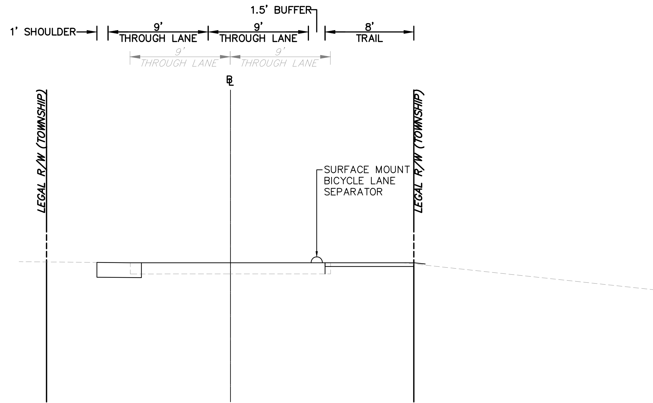
TYPICAL ROADWAY SECTION STATIONS VARY 8' TRAIL
