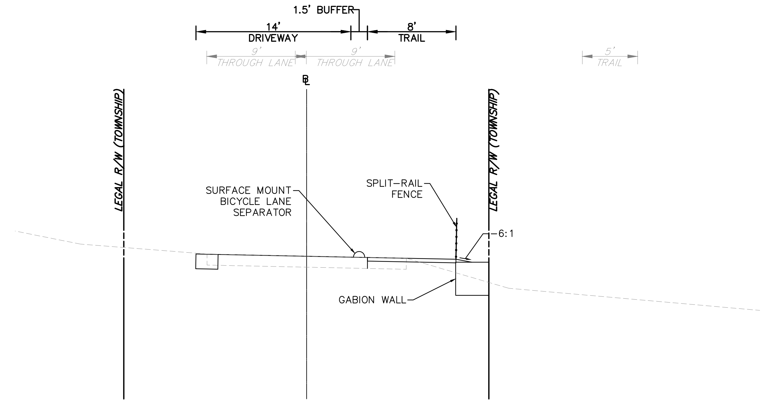
TYPICAL DRIVEWAY SECTION STA. 77+00 TO STA. 88+00 8' TRAIL
