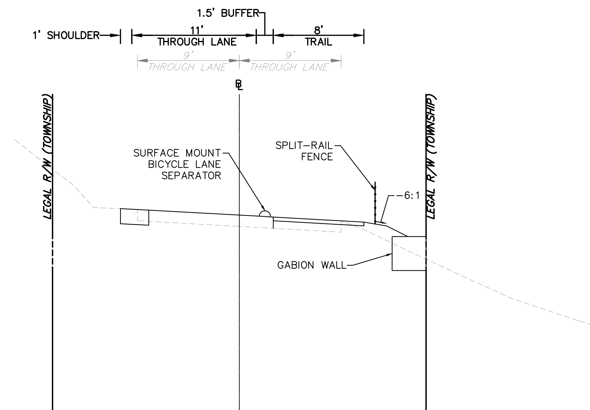
TYPICAL ONE-LANE CHOKER SECTION STA. 47+50 TO STA. 51+00 8' TRAIL
